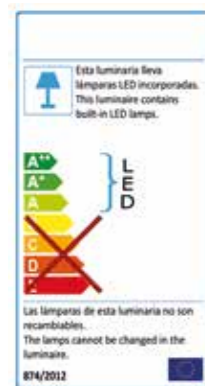
△ 148277 Puntos/points 380 Ø 42 ↓ 9 cm 22,5W LED 2.025 lumen / 3,000 K Peso/weight 1,38 Kg Medidas del florón Ø 42 ↓ 5,5 cm Sizes of the canopy
