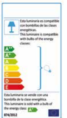
735953 △ Puntos/points 360 Ø 23 ↑ 55 cm 1 E27 LED 10W 900 lumen / 3.000 K Peso/weight 2,7 Kg
