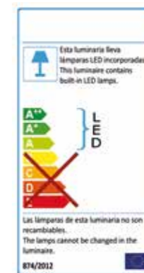
148193 △ Puntos/points 380 Ø 42 ↓ 9 cm 22,5W LED 2.025 lumen / 3,000 K Peso/weight 1,38 Kg Medidas del florón Ø 42 ↓ 5,5 cm Sizes of the canopy
