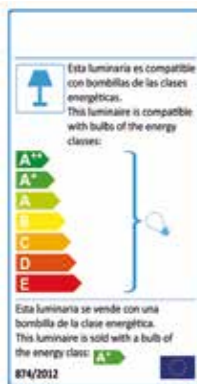
563710 Puntos/points 120 Ø 15 ↑ 43 cm 1 E27 LED 5,5W 450 lumen / 3.000 K Peso/weight 0,78 Kg
