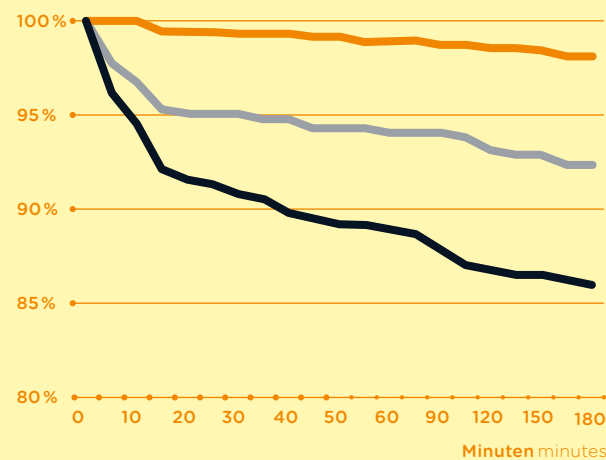
Deratingverhalten Derating behaviour
